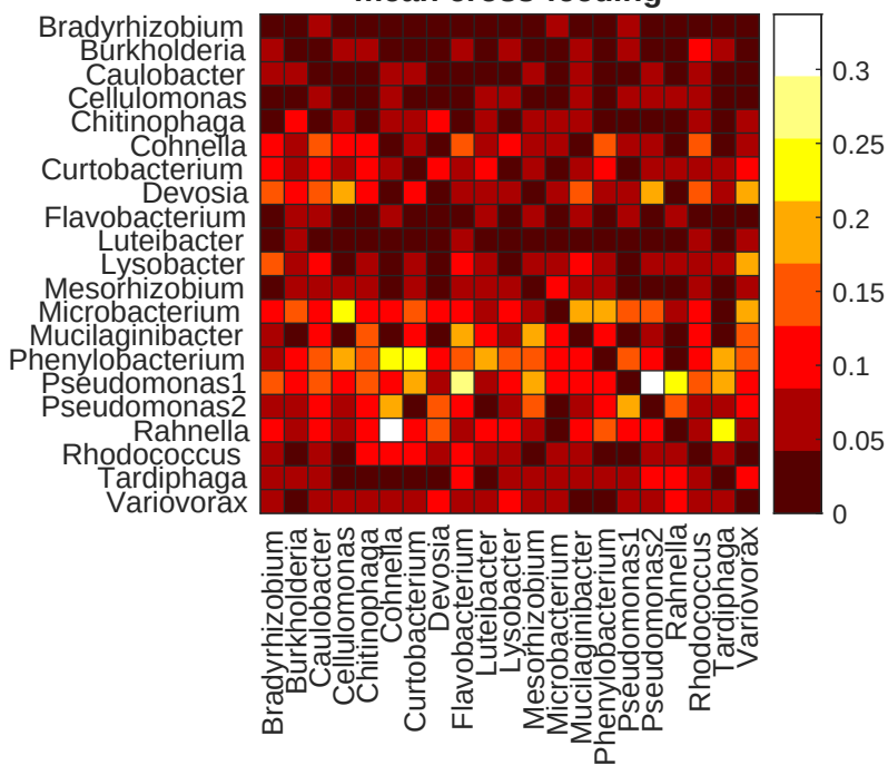
mean cross-feeding
